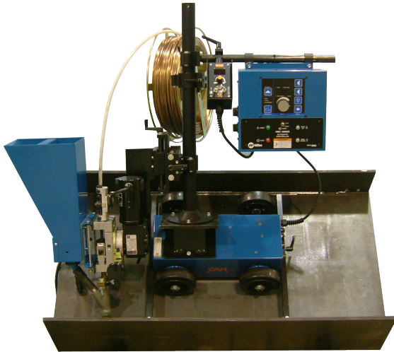
SAM® Submerged Arc Carriage... Shown set at 45° for beam welding application
