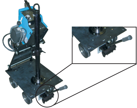
SAM® Heavy-Duty MIG Carriage... Shown supplied with optional steering mechanism and mast assembly
